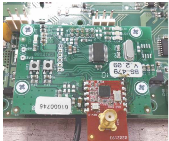
Figure 5 : Mounting of the board BS-479
