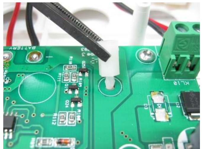
Figure 2 : Mounting of the spacers
